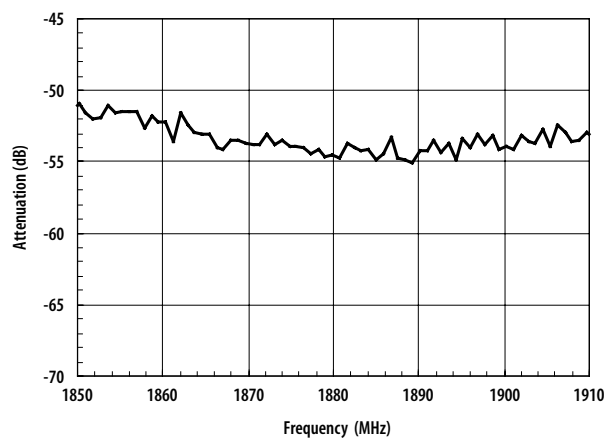
Figure 32. Isolation, PCS Tx Port to GPS Port in PCS Tx Band.
