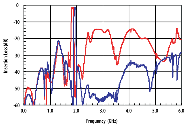
Figure 9. PCS Tx and Rx Wideband Insertion Loss.
