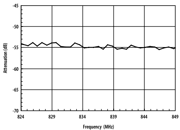
Figure 31. Isolation, Cellular Tx Port to GPS Port in Cellular Tx Band.
