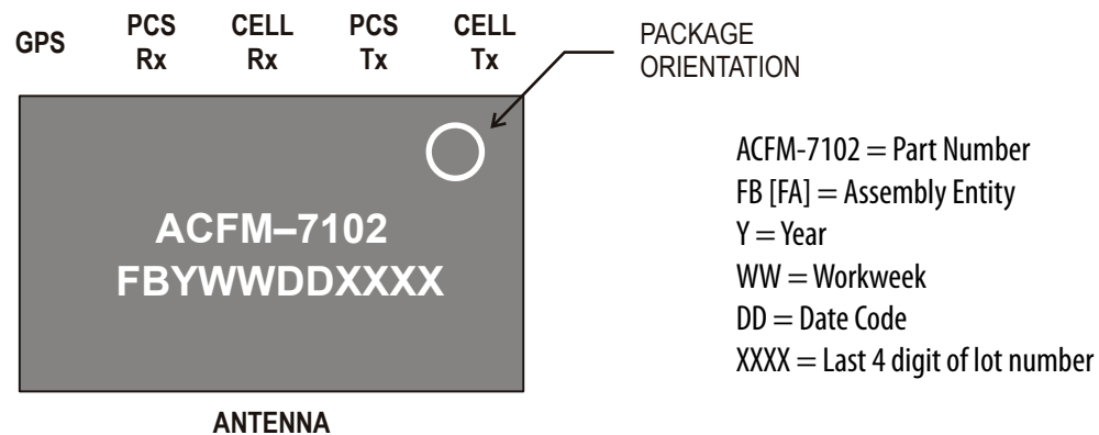
Figure 39. Package Marking.
