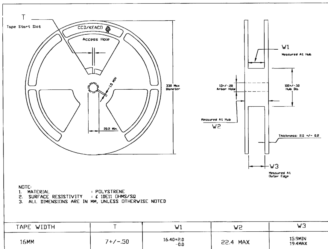
Figure 49. Reel Information.
