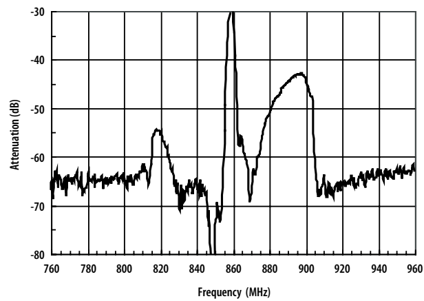
Figure 19. Cellular Tx-Rx Isolation.
